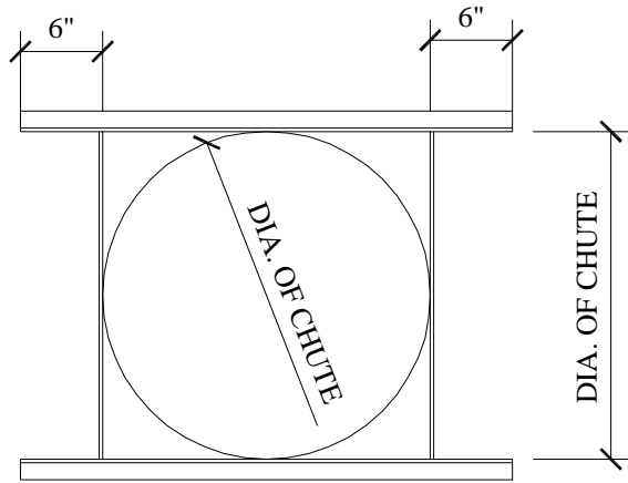
TYPICAL FLOOR FRAME
