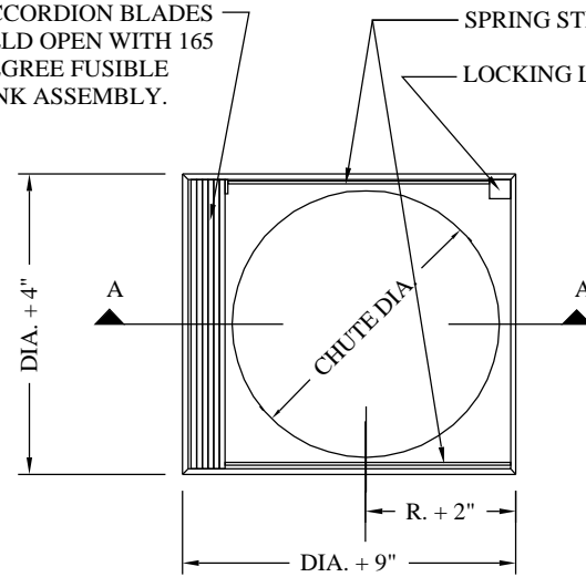
PLAN (INSIDE)
